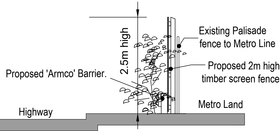
Typical Southern boundary detail. NTS.
